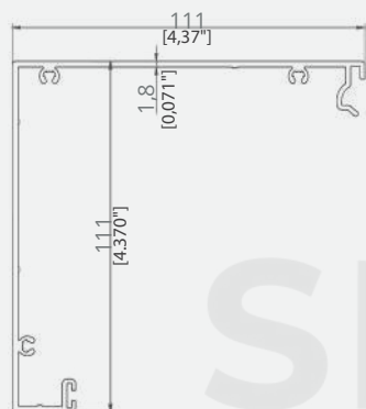
ENGINE BOX PROFILE
