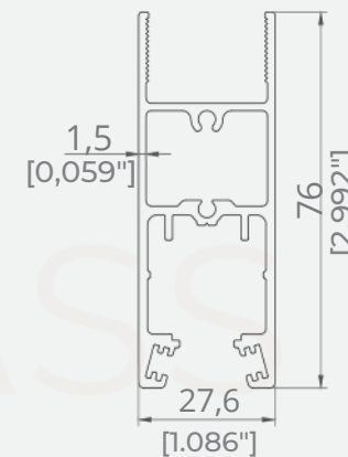
GLASS PANEL BASE PROFILE 22 MM
